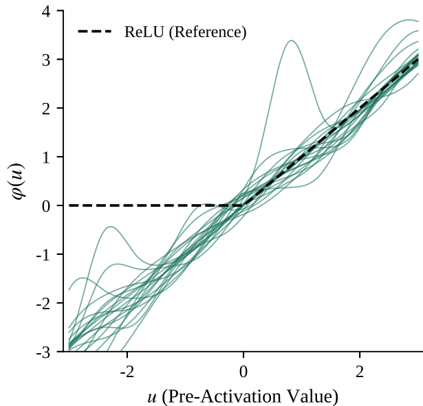
Smooth
