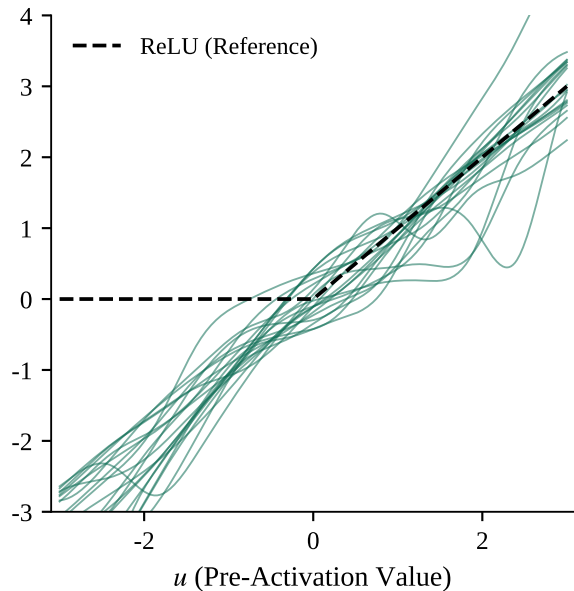
Piecewise Linear
