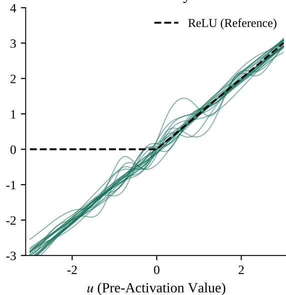
Oscillatory
